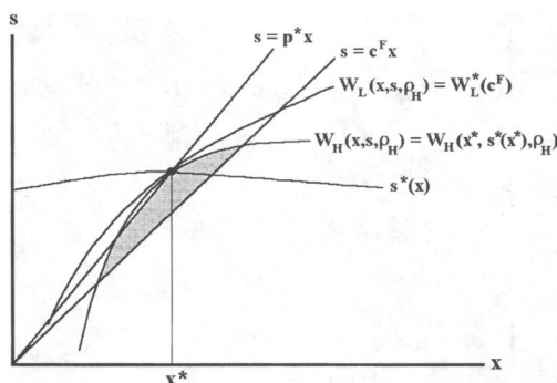
FIGURE 3. VEBLEN EFFECTS WITH THE TANGENCY PROPERTY
